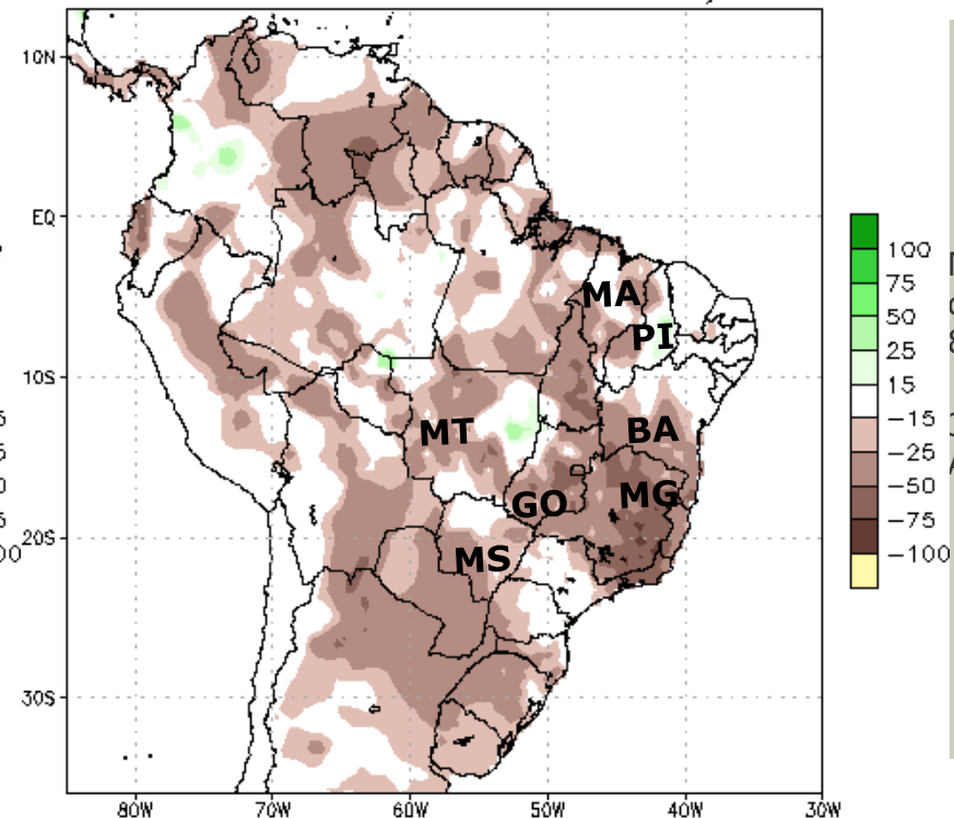
NCEP GFS Ensemble Forecast 8–14 Day Precipitation (mm) from: 24Jan2025 31Jan2025–06Feb2025 Anomaly
