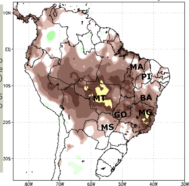
NCEP GFS Ensemble Forecast 1–7 Day Precipitation (mm) from: 24Jan2025 24Jan2025–30Jan2025 Anomaly
