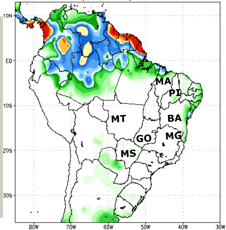
NCEP GFS Ensemble Forecast 1–7 Day Precipitation (mm) from: 13May2025 13May2025–19May2025 Accumulation
