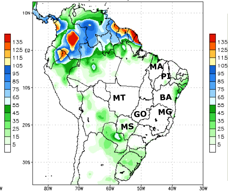
NCEP GFS Ensemble Forecast 8–14 Day Precipitation (mm) from: 13May2025 20May2025–26May2025 Accumulation
