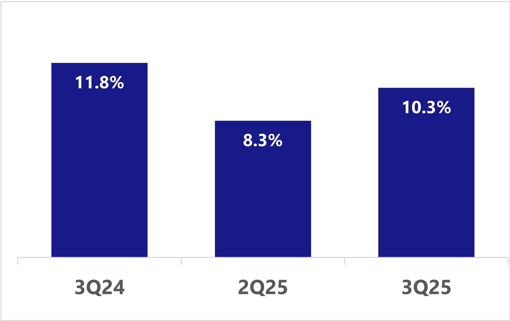
Churn
