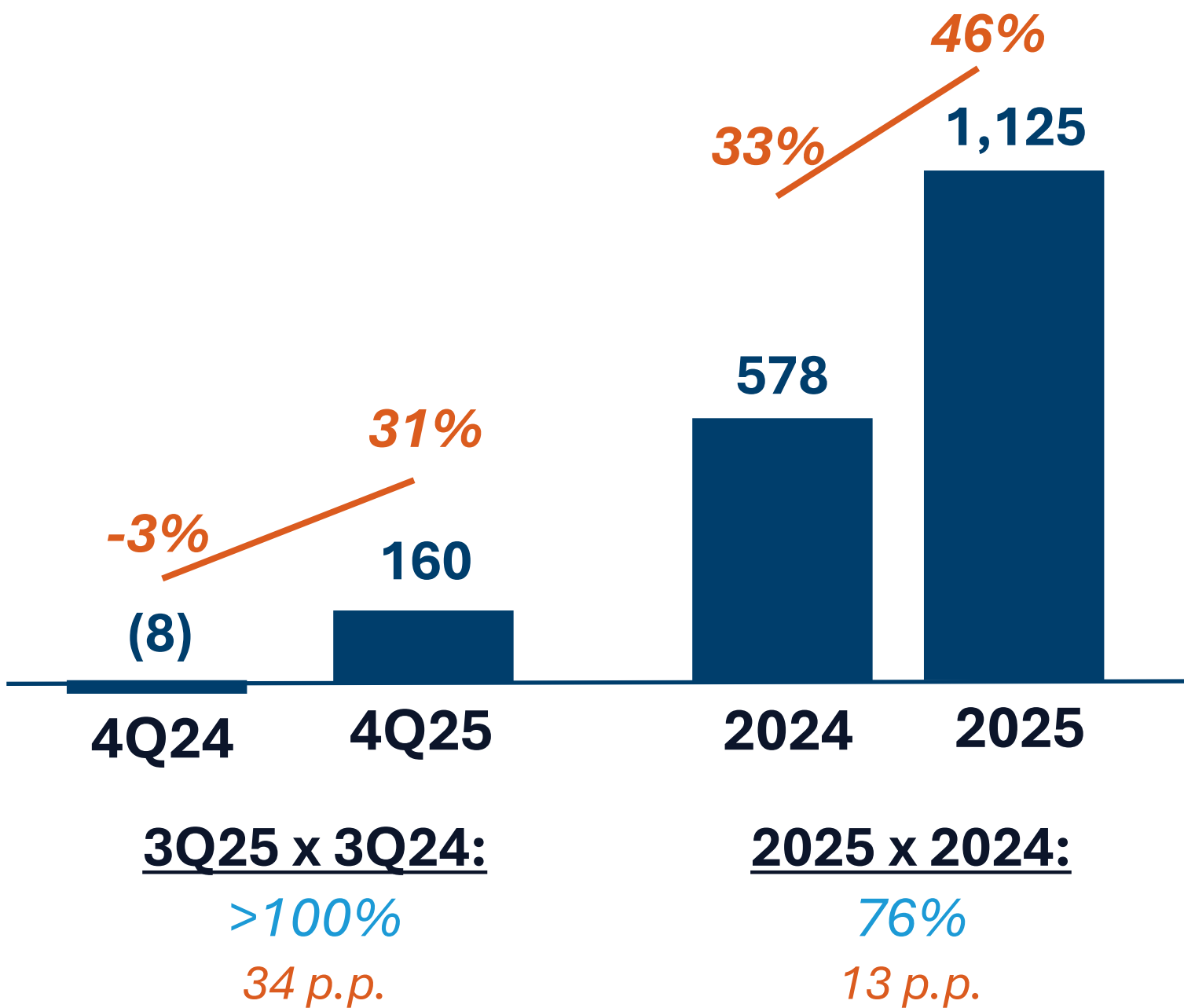
Recurring Adj. EBITDA (R$ million and EBITDA Mg.%)
